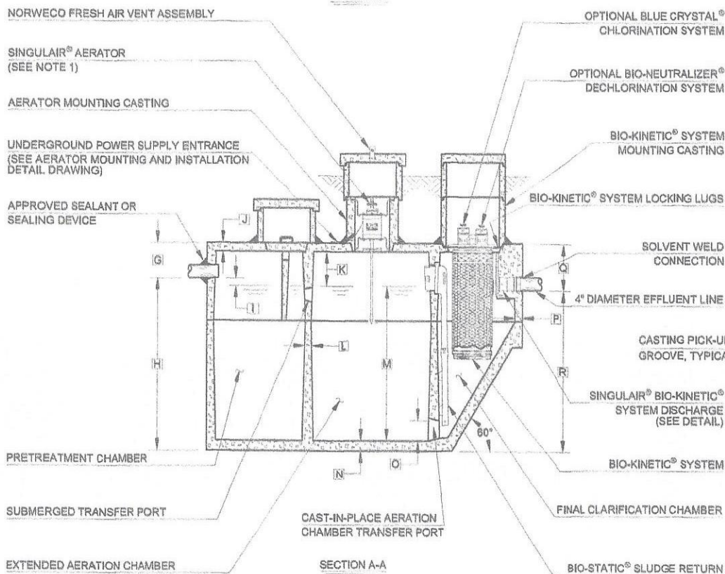
BIO-KINETIC® SYSTEM DISCHARGE DETAIL
